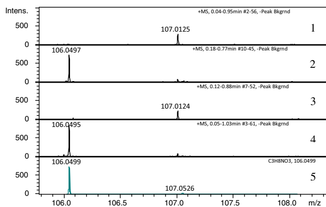
Fig. 4. Spectra of decarboxylation of aspartic acid. (1) Sample maintained in the dark at the DLR; (2) sample exposed to UV light at the DLR; (3) sample maintained in the dark on the ISS; (4) sample exposed to sun on the ISS and (5) theoretical spectrum of C_3H_8NO_3^+ .
