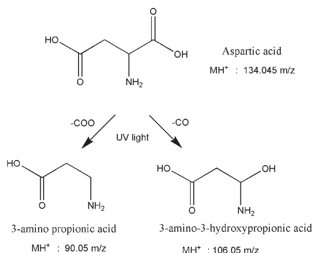
Fig. 5. Proposition of the aspartic acid photoalteration processes: decarboxylation of aspartic acid into 3-aminopropionic acid ( \beta -alanine) and decarboxylation of aspartic acid into 3-amino-3-hydroxypropionic acid.
