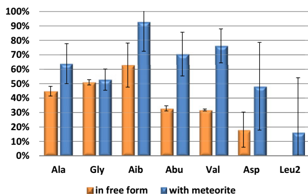
Fig. 2. Rate of remaining compounds measured after exposure in samples exposed to UV in comparison with samples maintained in the dark with or without meteorite powder in DLR laboratory.
