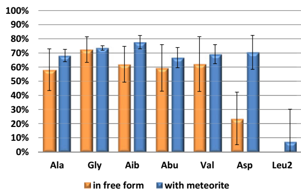
Fig. 3. Rate of survival of compound measured after exposure in samples exposed to UV in comparison with samples maintained in the dark with or without meteorite powder in the AMINO experiment on ISS.
