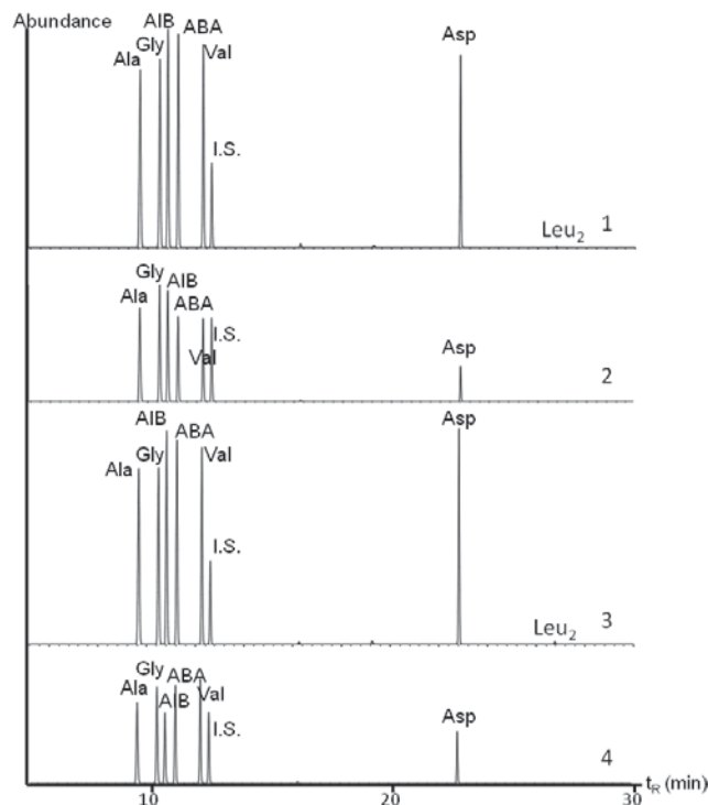
Fig. 1. Chromatograms in SIM mode of silylated extracts analysed on the CP-Sil 19 CB column of (1) a control of the DLR (2) a sample exposed of the DLR (3) a flight dark control of the ISS and (4) a sample exposed on the ISS.
