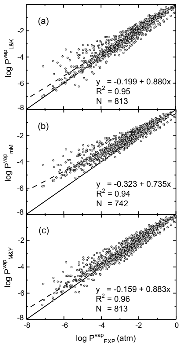
Fig. B.2 Estimated P^{vap} versus experimental values for the (a) L&K, (b) mM and (c) M&Y methods. The continuous and dashed lines are respectively the y = x and regression lines.
