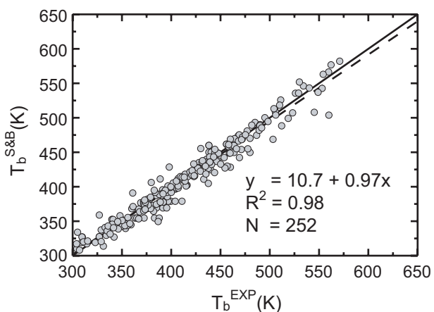
Fig. B.1. Boiling points estimated with the Stein and Brown method (Stein and Brown, 1994) versus experimental values. The continuous and dashed lines are respectively the y = x and regression lines.
