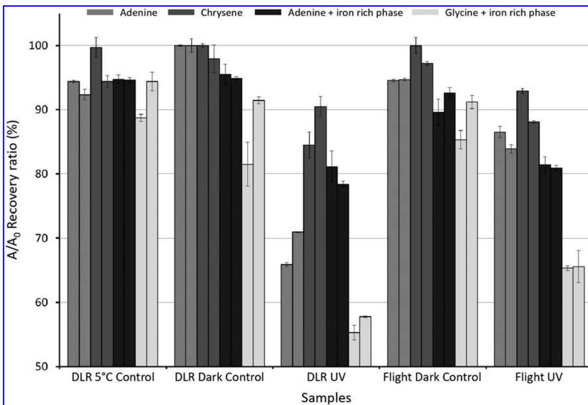
FIG. 8. A/A_0 recovery ratio of the DLR (5°C, dark control, UV exposed) and PSS (flight dark control, flight sun-exposed) samples calculated from FTIR spectra. In gray, adenine; in dark gray, chrysene; in black, adenine + iron-rich phase; in light gray, glycine + iron-rich phase.
